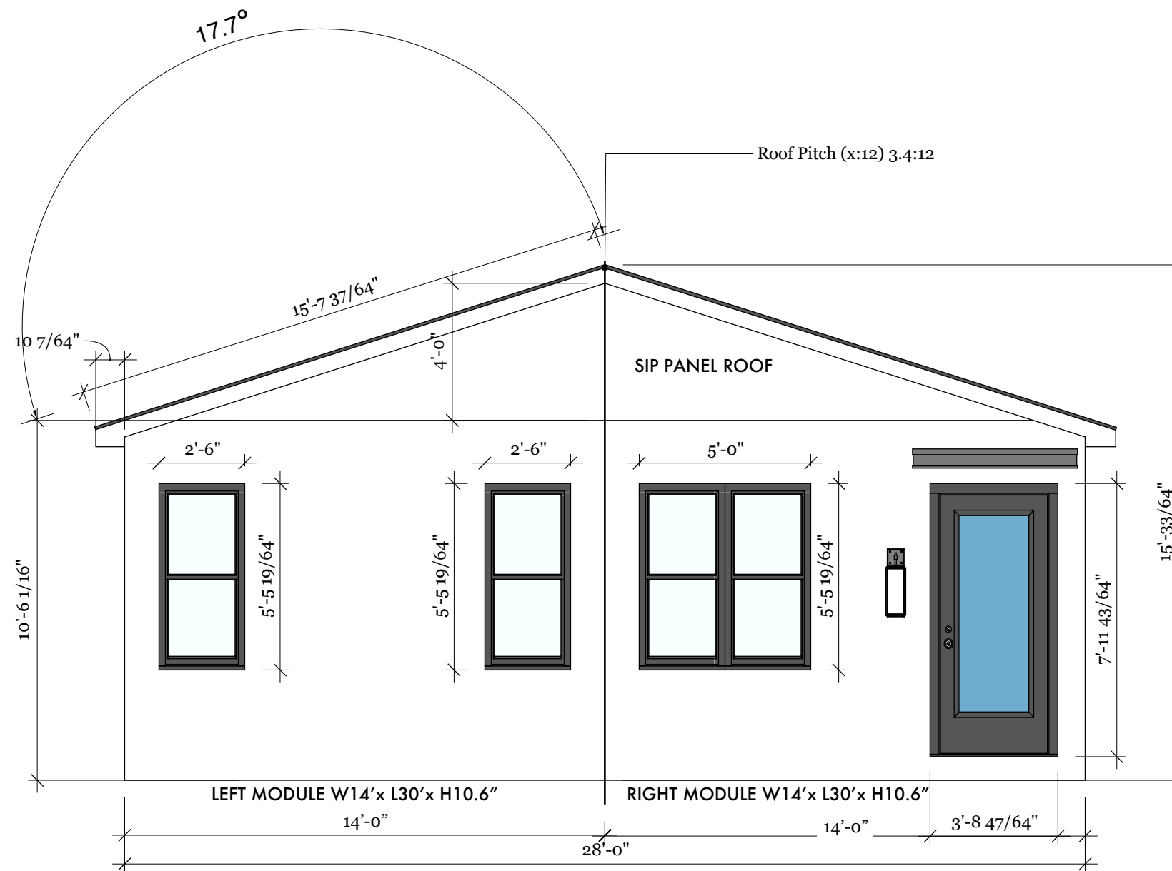
FRONT ELEVATION
